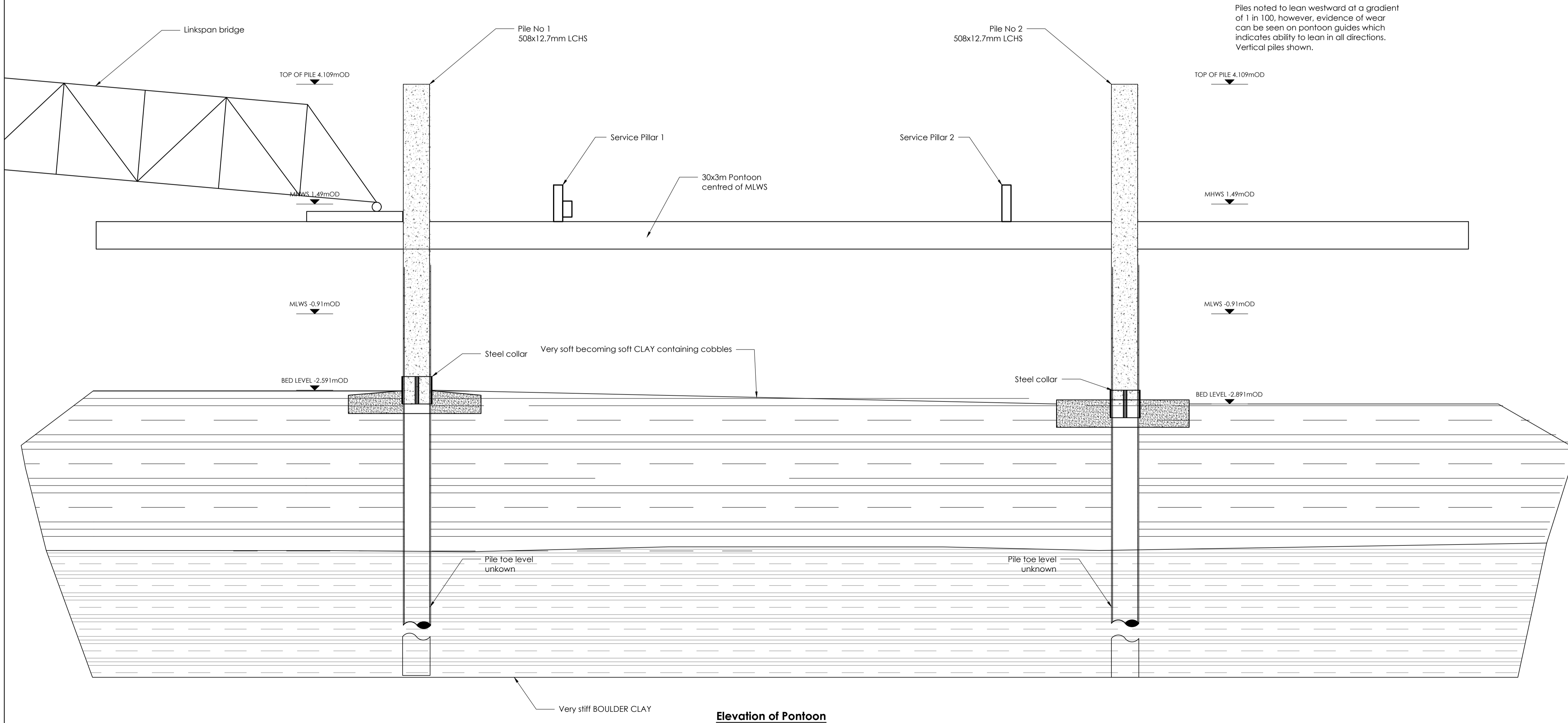
Elevation of Pontoon Scale 1:50
