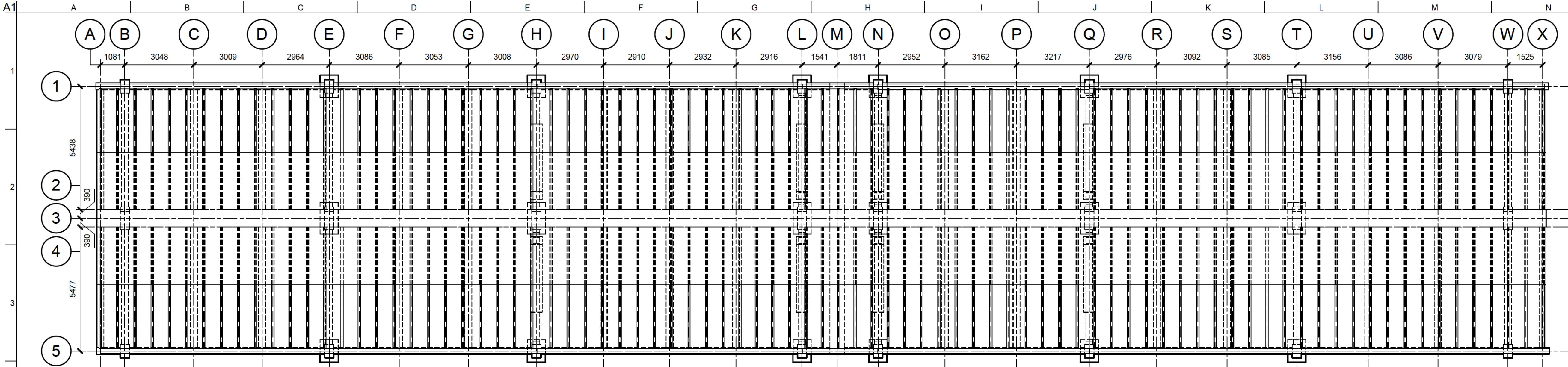
Upper Deck Scale 1 : 100
