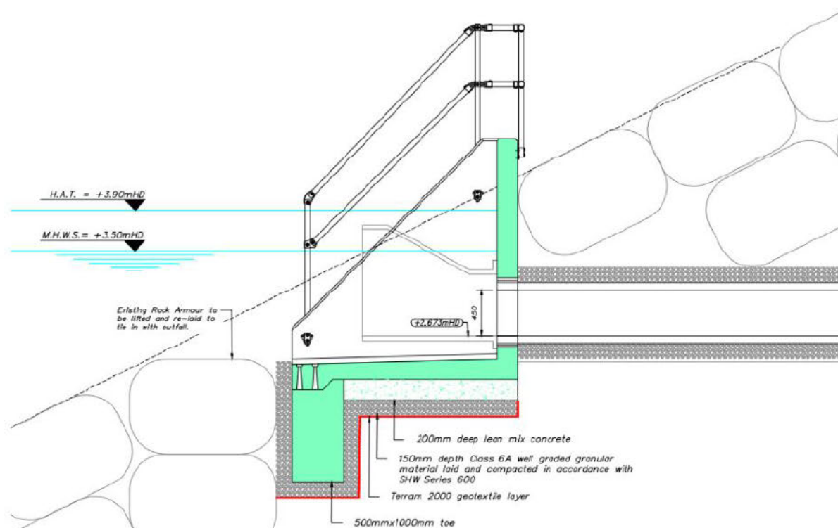
Figure 2-1: Cross-section of outfall through quay wall
