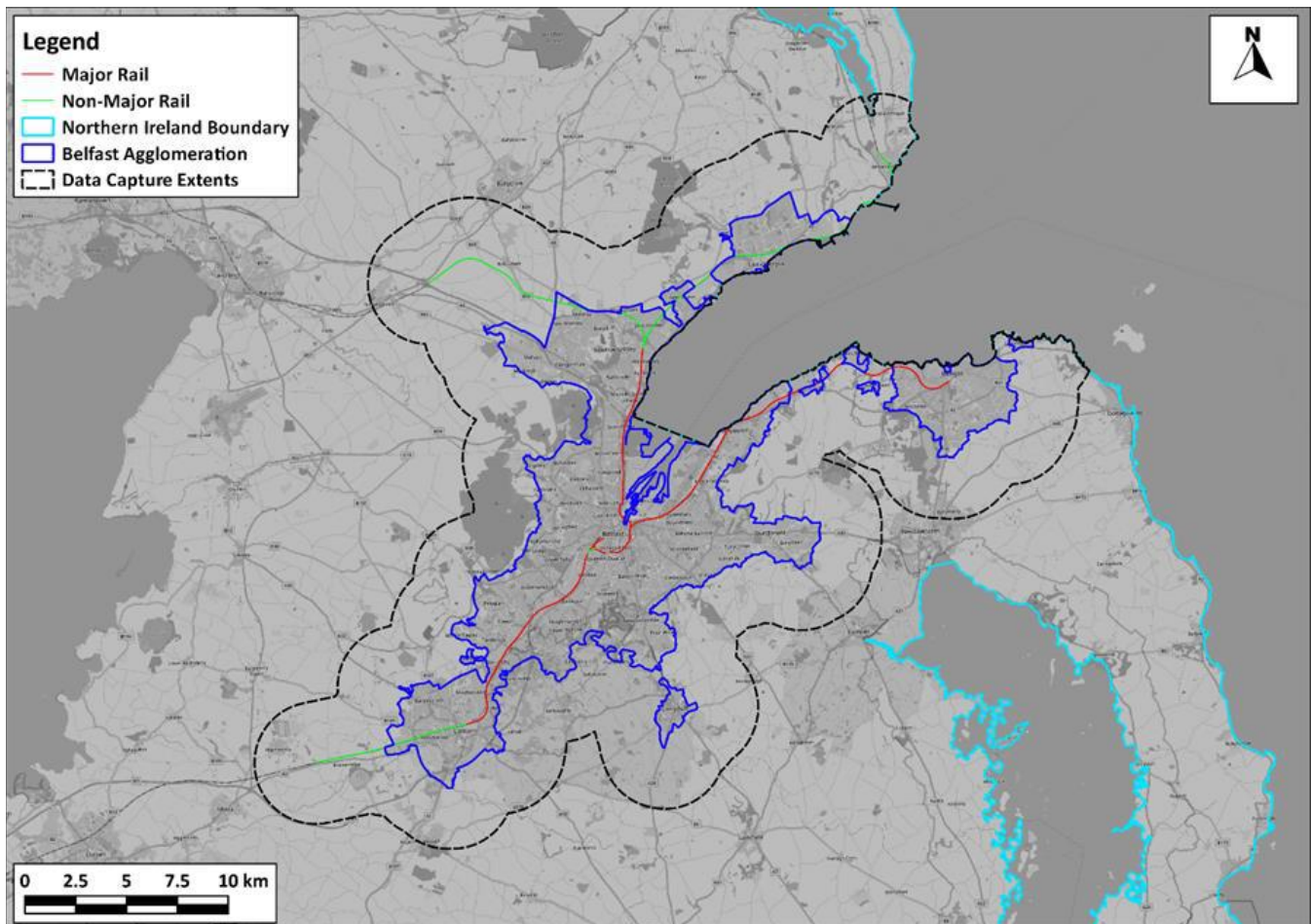
Plate 3.1 Belfast Agglomeration Boundary and Major/Non-Major Railway Calculation Extents, Round Four
