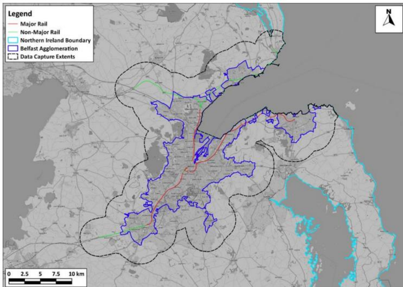
Plate 5.1 Rail Model Data Capture Extents, Round Four
