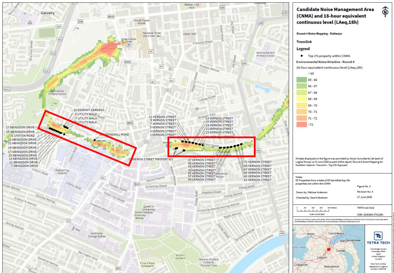
Plate 6.2 Candidate Noise Management Areas Rail and Top 1% Properties (>50 dB LAeq,18h)
