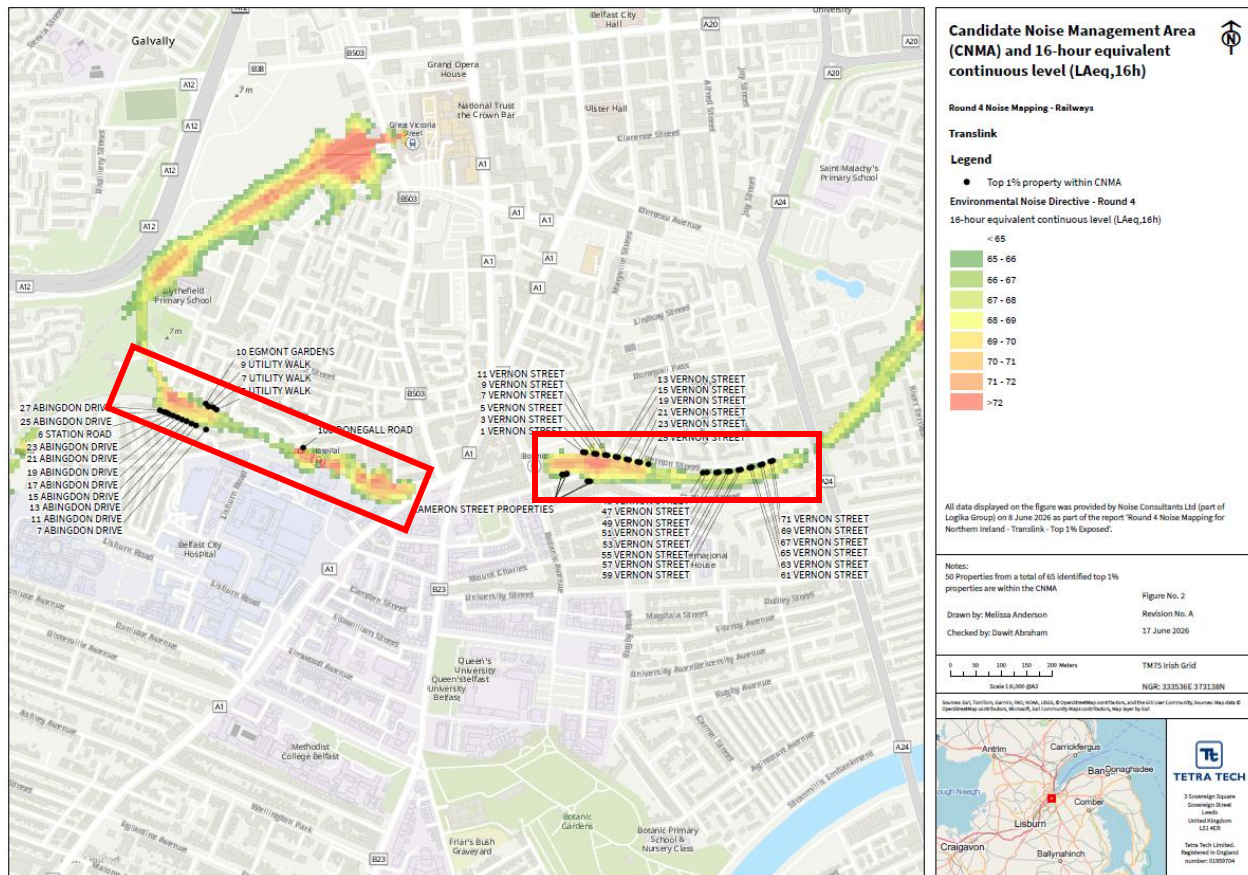
Plate 6.3 Candidate Noise Management Areas Rail and Top 1% Properties (>50 dB LAeq,16h)
