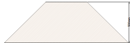
Compacted Clay Engineered Bund
