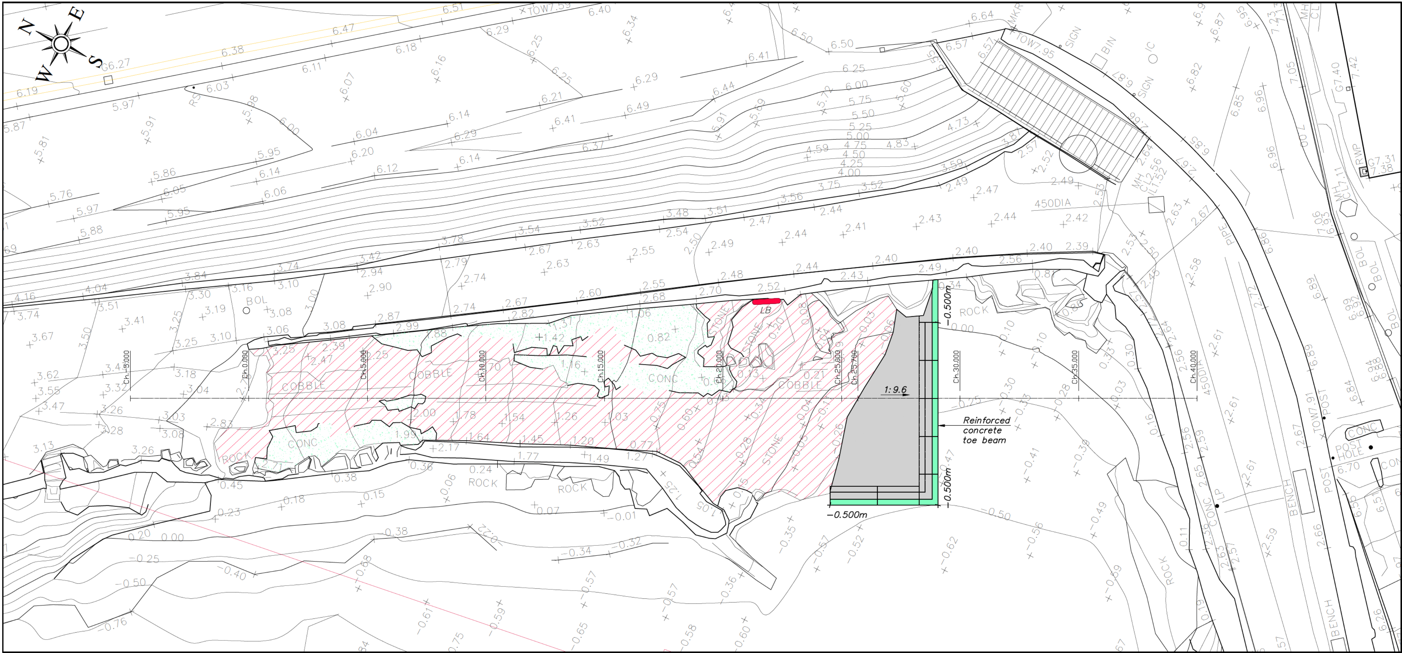
Proposed Slipway Plan 1:100
