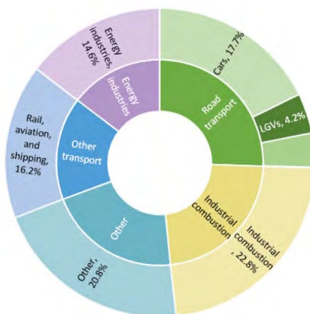
Figure 2-3 - NO 2 emissions in Northern Ireland 2017
