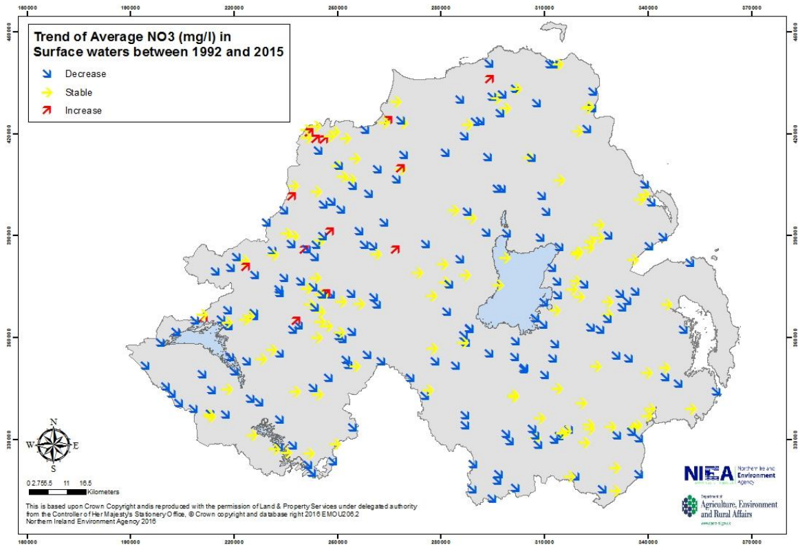
Figure 1.14: Overall trend of average nitrate ( \text{NO}_3 mg/l) in surface waters across Northern Ireland in the period January 1992 to December 2015
