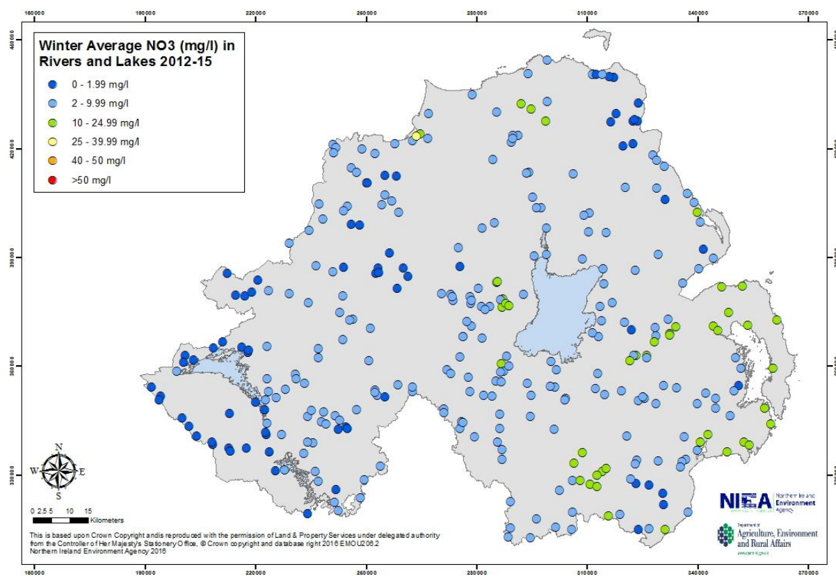
Figure 1.9: Annual winter nitrate concentrations (NO 3 mg/l) in rivers and lakes, 2012–2015
